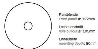
Dimensions and drilling distances ILD (self-contained / CBS)
